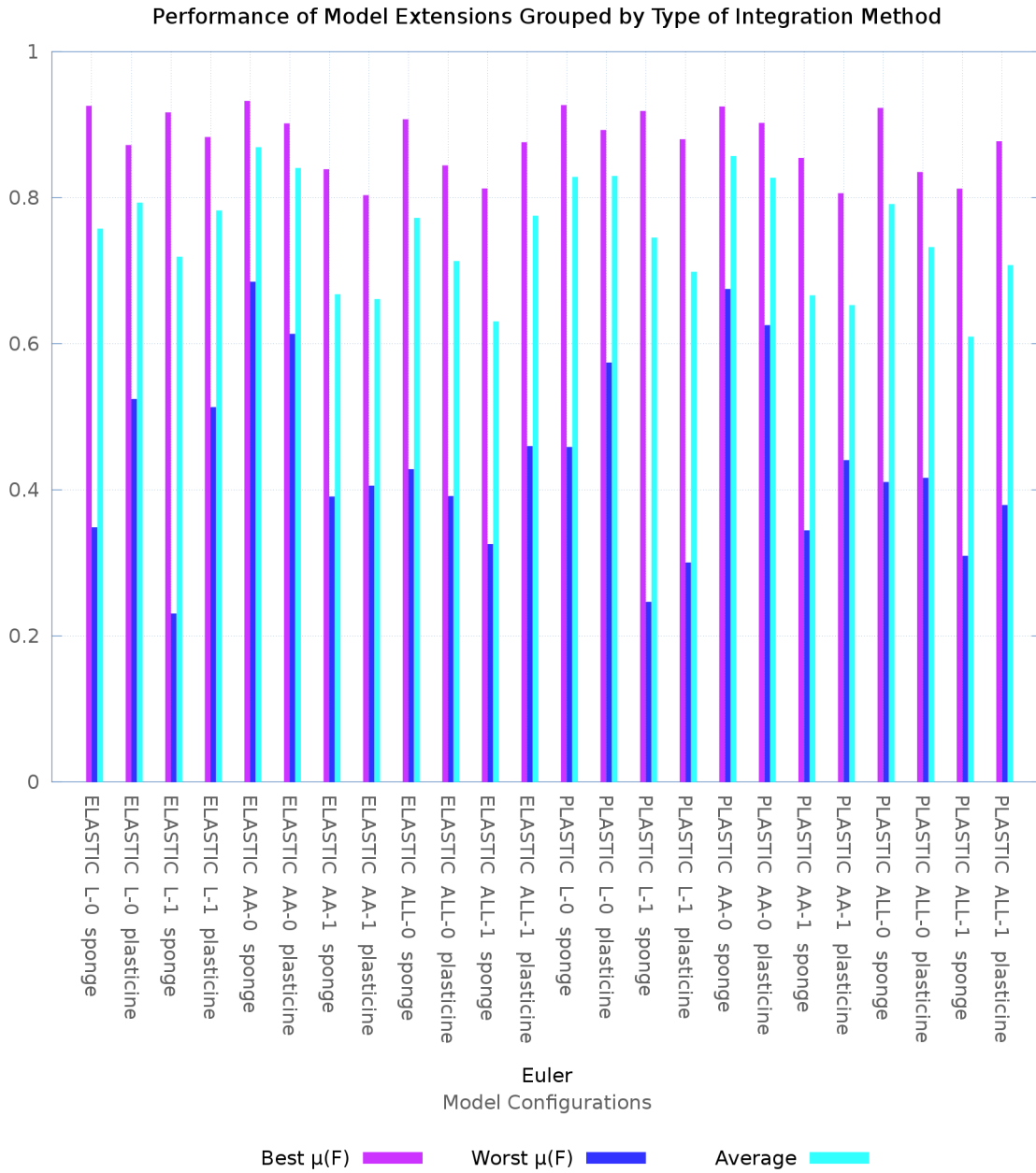
FIGURE 10.2: Best, worst and average mark for each variation of the mass-spring model as explained in Table 10.1, when trained for the sponge and plasticine (putty), with the Euler integration scheme.
