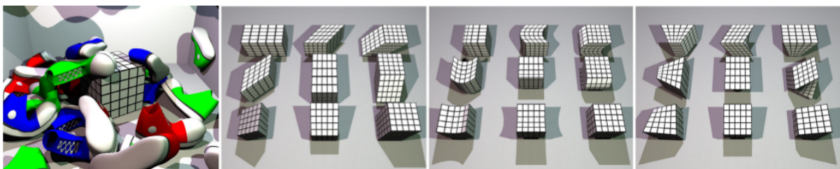
FIGURE 7.8: Shape matching with geometrically inspired modes. The linear shear and stretch modes and the quadratic bend and twist modes are shown. Taken from [56], with permission.
