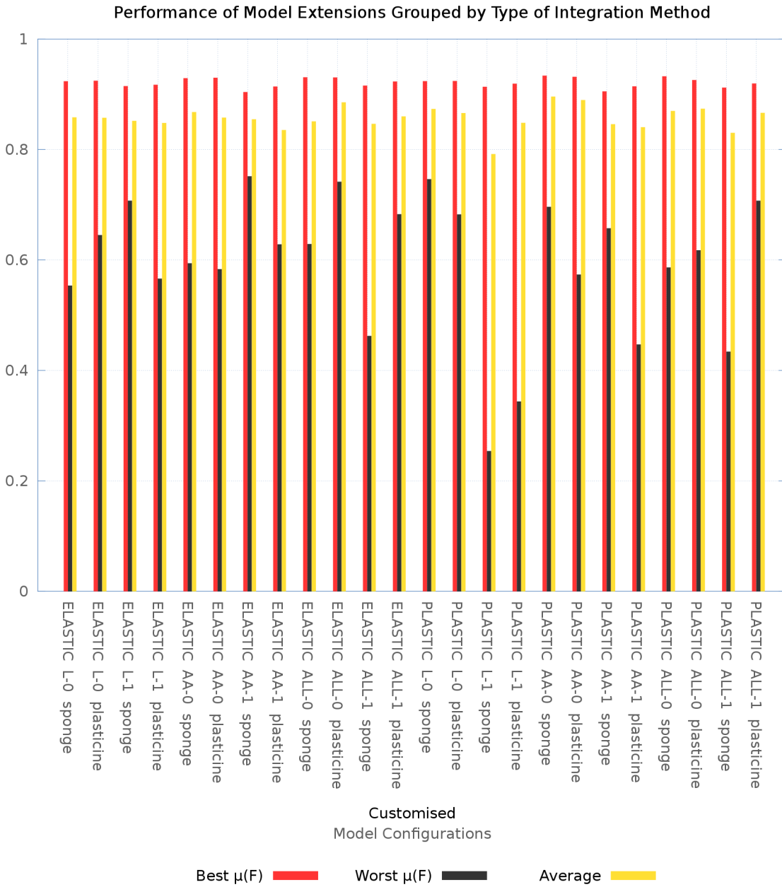
FIGURE 10.4: Best, worst and average mark for each variation of the mass-spring model as explained in Table 10.1, when trained for the sponge and plasticine (putty), with our customised equations.
