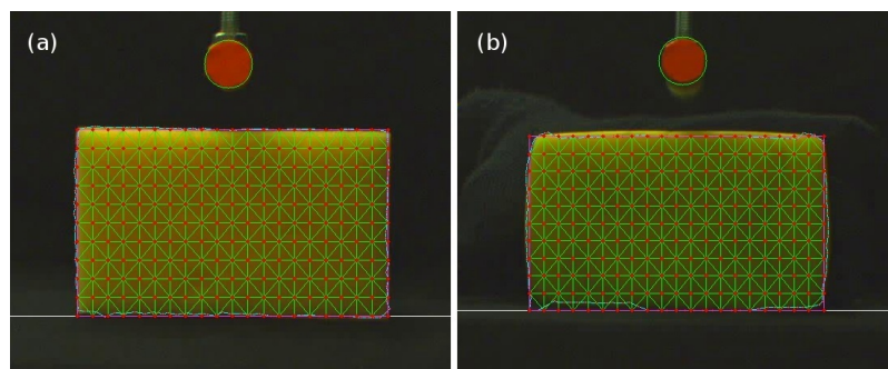
FIGURE 10.1: Initial mesh for the (a) sponge and (b) plasticine.
