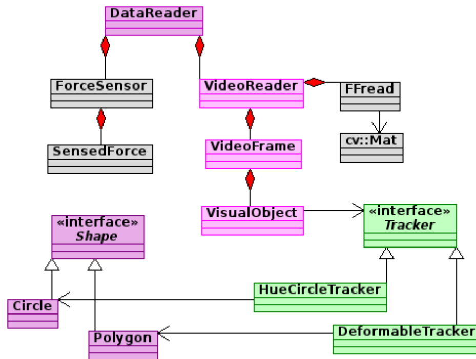
FIGURE A.2: UML diagram of the package in charge of reading the information from the sensors and interpret it as forces and shapes.
