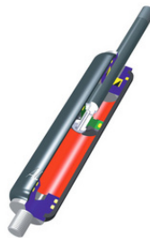
FIGURE 5.11: Hydraulic damper. [Taken from the web.]
