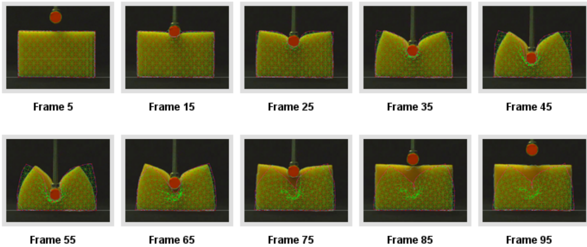
FIGURE 10.11: Training data.
