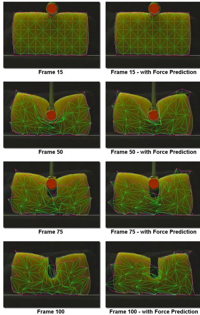
FIGURE 10.25: Simulation of the plasticine. Comparison of the images generated without and with force prediction, simulating with geometric collision recovery routines.
